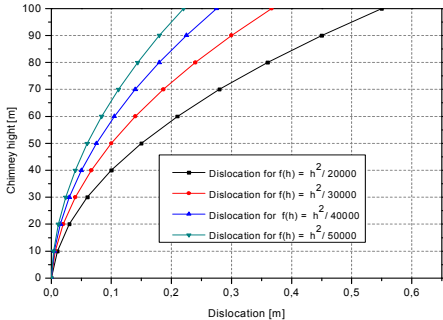
Fig.6. Dislocations of vertical axis described by parabolic function
