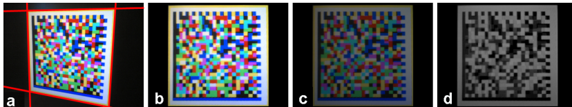
Fig. 4. Preprocessing steps for decoding: (a) captured frame and detected corners, (b) rectified image, (c) contrast and brightness adjusted image, (d) extracted 2D barcode (red channel) in gray scale.
