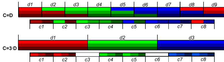
Fig. 3. Encoding: sifted (top) and non-shifted (bottom) encoding scheme ( c_i and d_i are captured and displayed frames respectively, the individual frame-embedded and captured/transmitted barcodes are color-coded).
