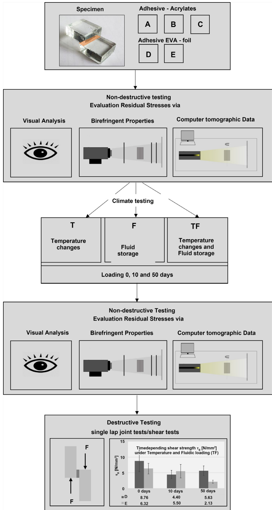
Figure 2. Experimental approach for the evaluation of long-term behavior of bonded glass panes.
