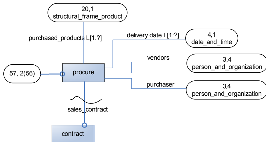
Figure 7: Section of the LPM/5-EXPRESS-G CIS/2 diagram for “procure”
